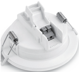
Tool less loop-in/ Out push fit Terminal
